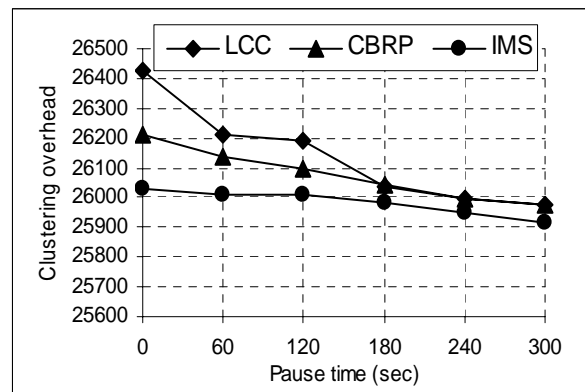
Figure 4 clustering overhead vs. pause time
