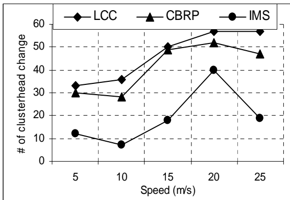
Figure 5 Number of clusterhead change vs. speed
